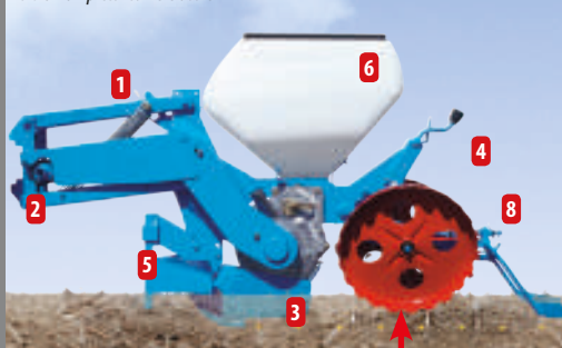
Depth control with rear wheels
